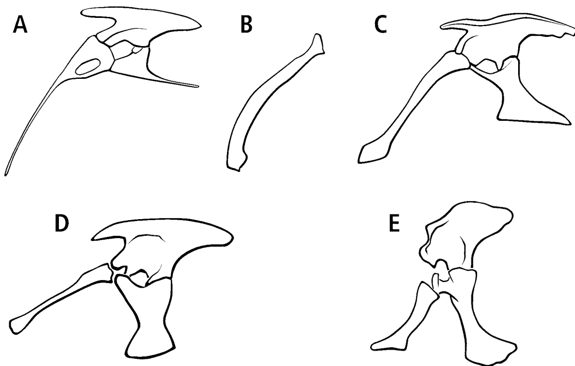
FIGURE 7. Lateral views of the pelvic girdles of selected Crocodylomorpha. A, Terrestrisuchus gracilis (Crush 1984). B, Hesperosuchus (Parrish 1991). C, Protosuchus richardsoni (Colbert and Mook 1951). D, Orthosuchus stormbergi (Nash 1968). E, Alligator (Romer 1956).
