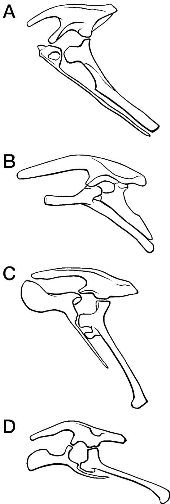
FIGURE 11. Lateral view of the pelvic girdles of selected ornithischian dinosaurs. A, The basal ornithischian Leiothorax diagnosticus (Thulborn 1972; Santa Luca 1984; Weishampel and Witmer 1990a). B, Stegosaurus (Gilmore 1914; Ostrom and McIntosh 1966; Galton 1990). C, The iguanodon Ouranosaurus nigeriensis (Taquet, 1976; Norman and Weishampel 1990). D, The hadrosaur Corythosaurus casuarius (Brown 1916; Weishampel and Horner 1990).
