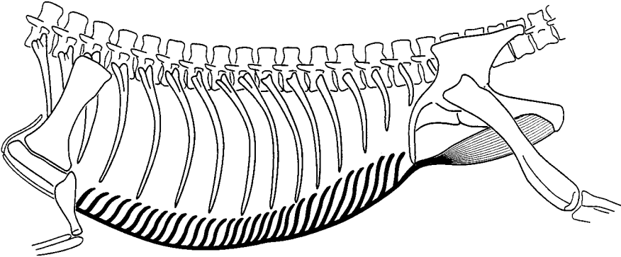
FIGURE 5. Illustration of proposed cuirassal breathing mechanism in the archosauromorph Euarkeria capensis . During expiration, contraction of the rectus abdominis muscle pulled the medial portion of the gastralia anteriorly, causing an elevation of the ventral body wall. During inspiration, contraction of the ischiotruncus muscle pulled the medial portion of the gastralia posteriorly, causing a depression of the ventral body wall and an increase in the volume of the body cavity. Modified from Ewer 1965.
